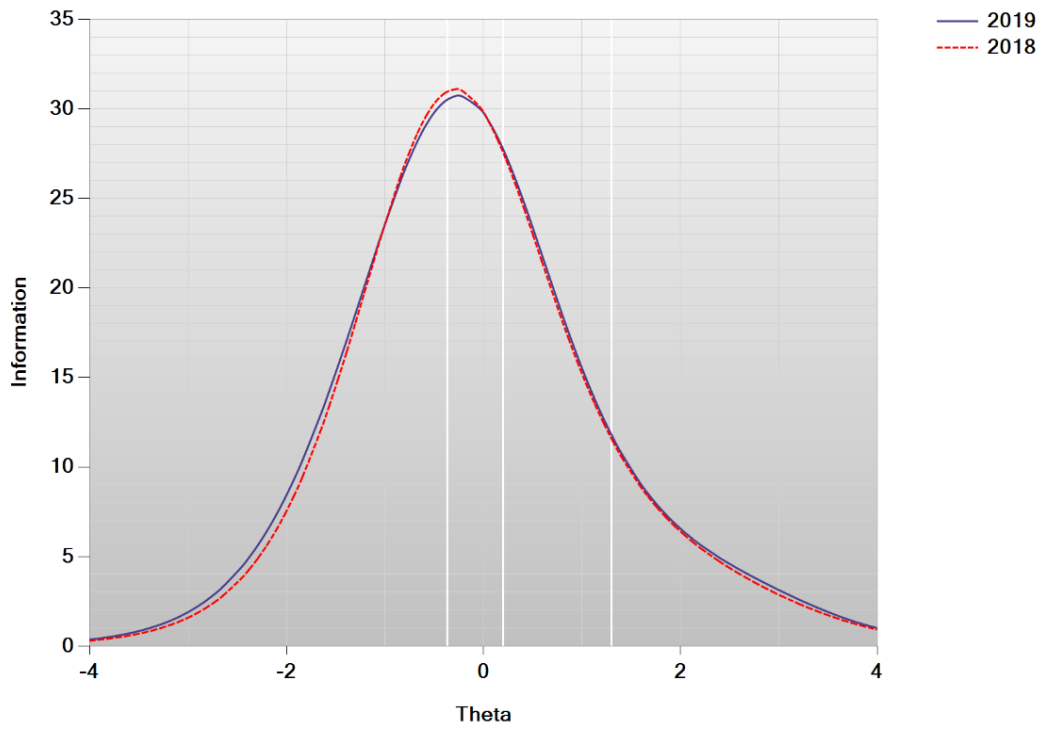
Figure L-8. Test Information Function – High School Technology/Engineering
