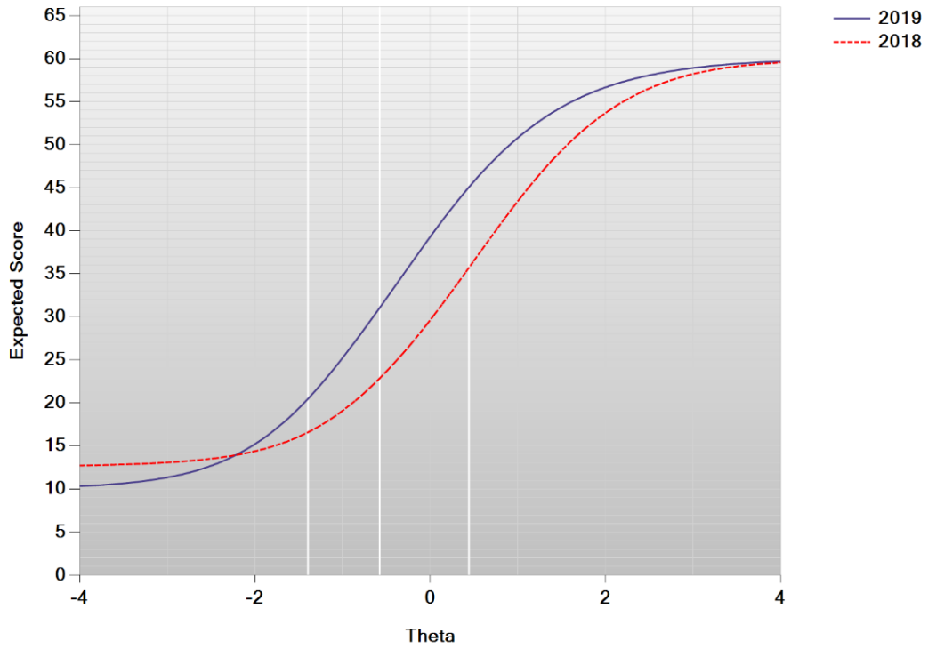
Figure L-5. Test Characteristic Curve – High School Introductory Physics
