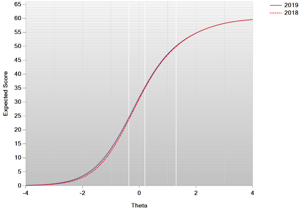
Figure L-7. Test Characteristic Curve – High School Technology/Engineering
