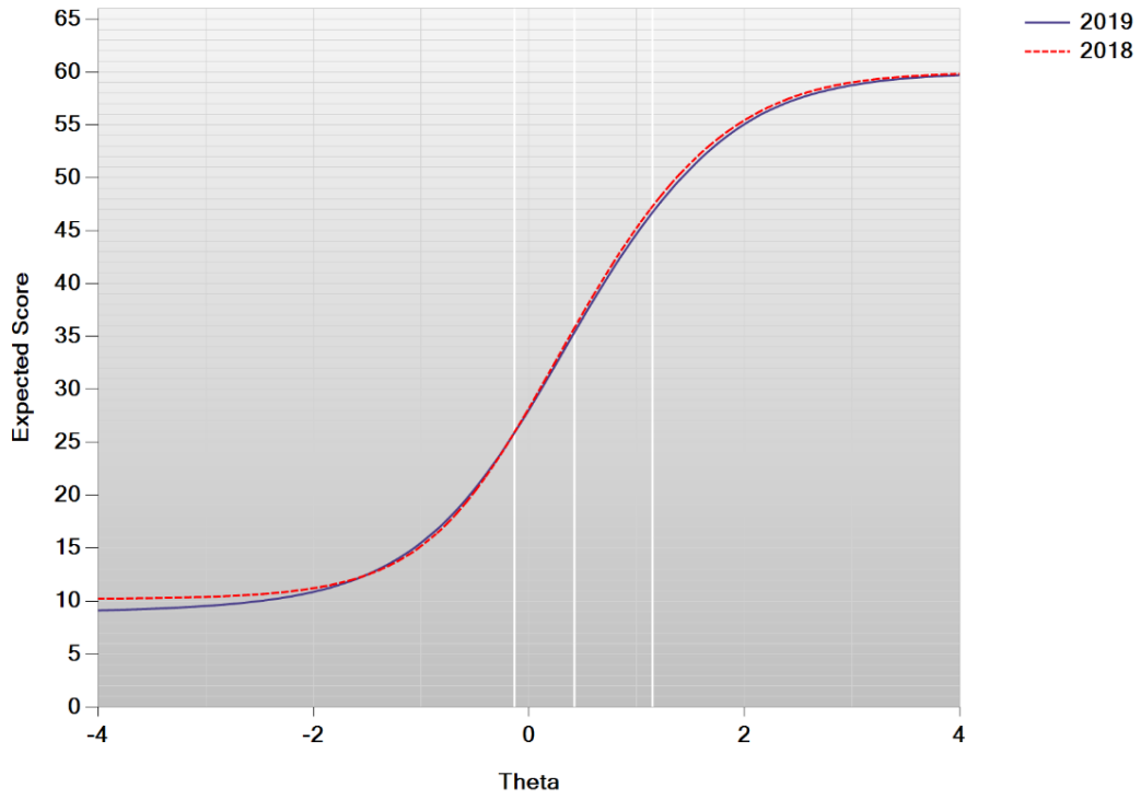
Figure L-3. Test Characteristic Curve – High School Chemistry
